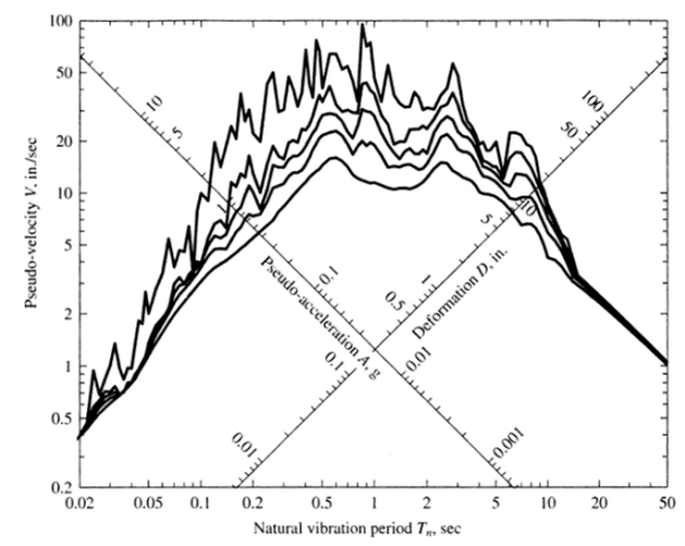
Combined D - V - A response spectrum, El Centro 1940 NS record, for 0 \leq \zeta \leq 20\% and full range of periods.
